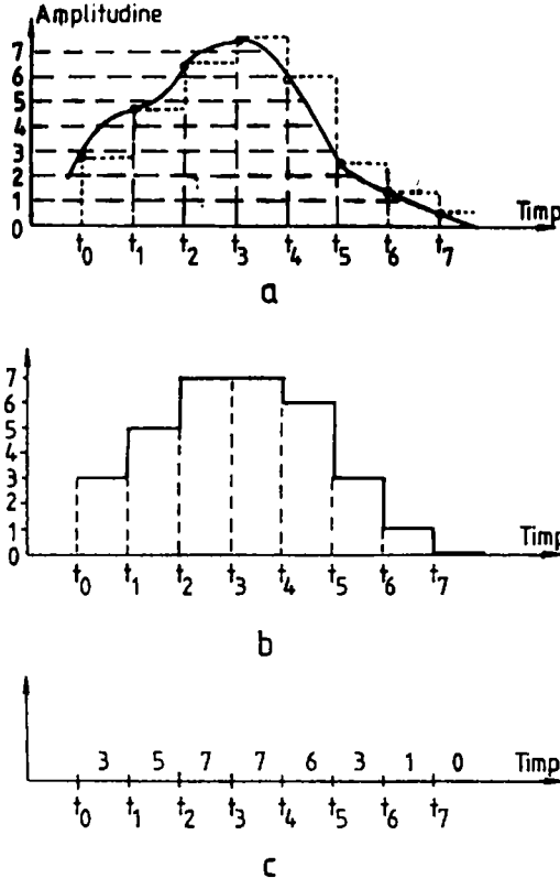
Fig. 2.2 Semnal digital:
